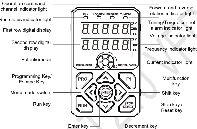
Figure 4-1 Operation panel
