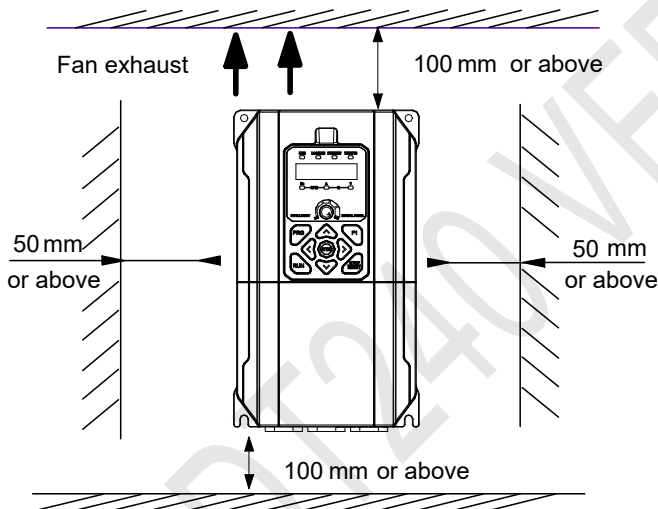
Figure 3-1 Installation spacing distance
